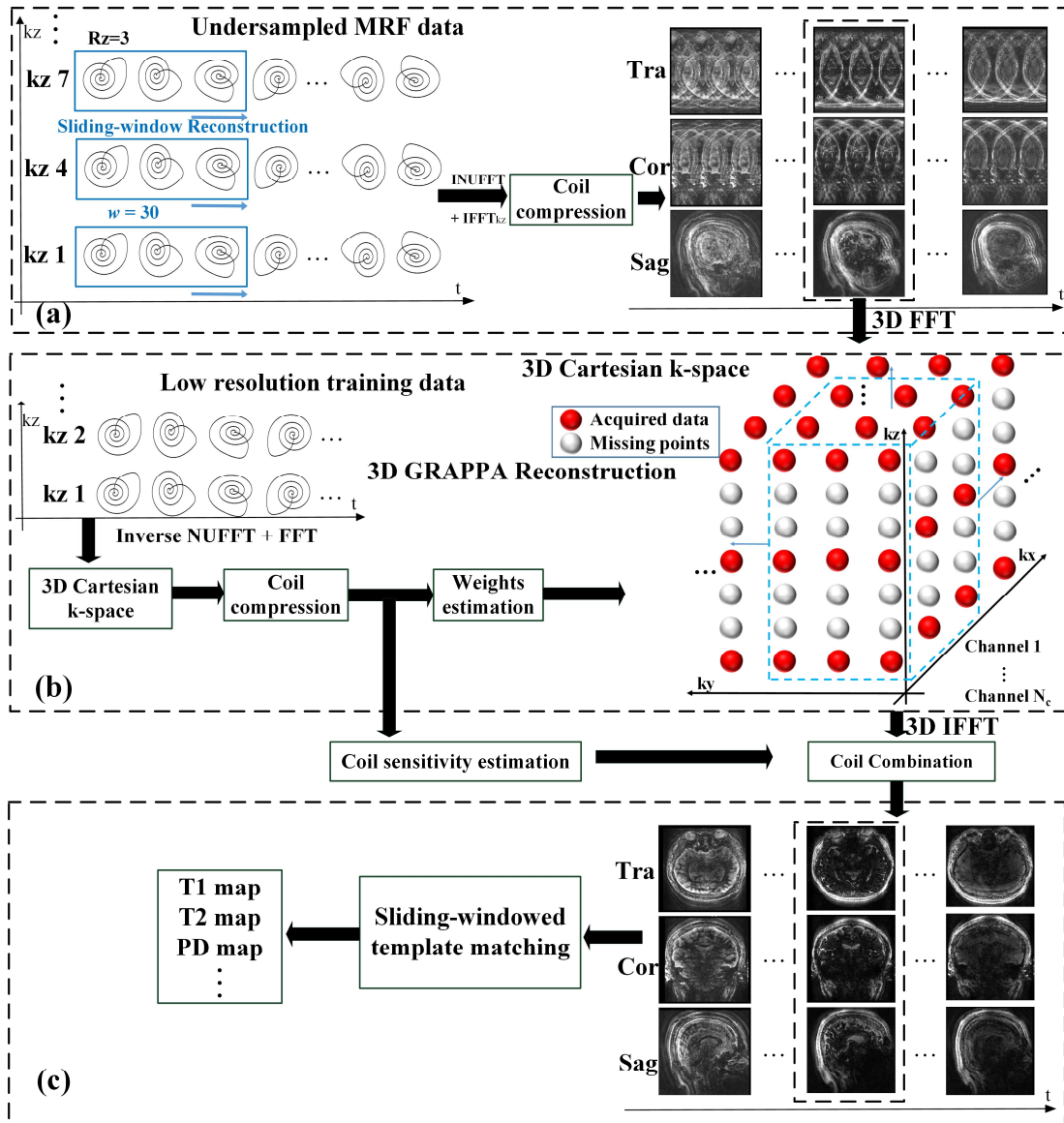
Fig.2. Hybrid of sliding-window and 3D GRAPPA reconstruction strategy. (a) sliding-window reconstruction was used for every partition of under-sampled MRF data, and transformed to Cartesian k-space after geometry coil compression. (b) 3D GRAPPA reconstruction. The acquired training data were utilized for coil sensitivity and 3D GRAPPA kernel estimations. Then the trained GRAPPA weights were applied on under-sampled Cartesian k-space and the sensitivity maps were used for coil combination. (c) The final T_1 , T_2 and PD maps were obtained by sliding-windowed dictionary recognition from aliasing-free volumes.
